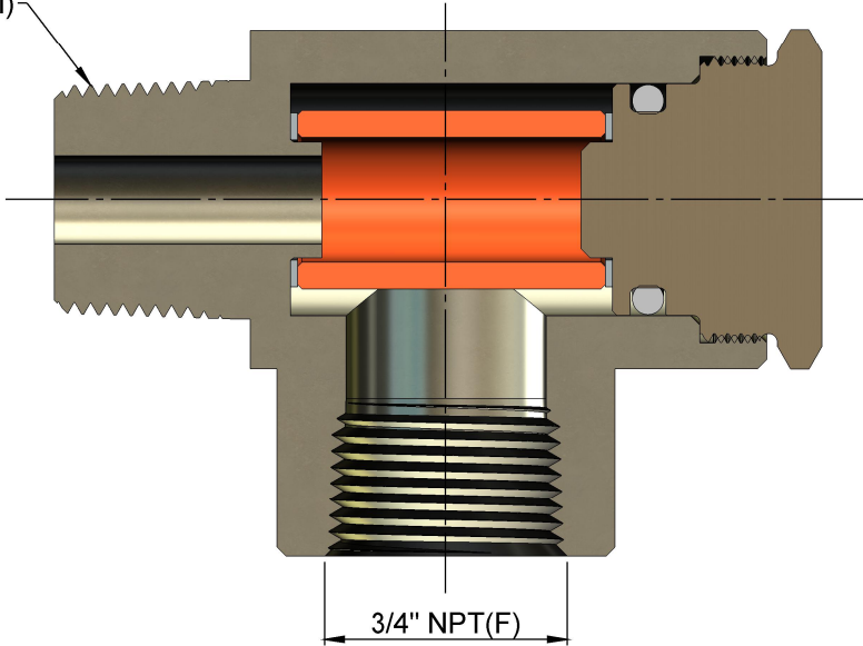
SECTIONAL VIEW
