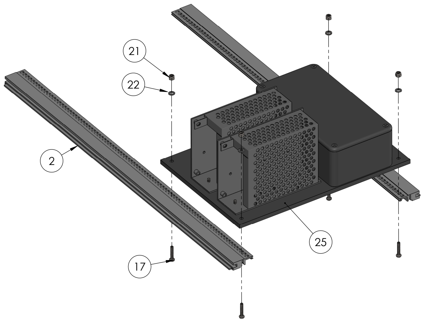
PSU'S & MOUNTING/PROTECTING COMPONENTS
