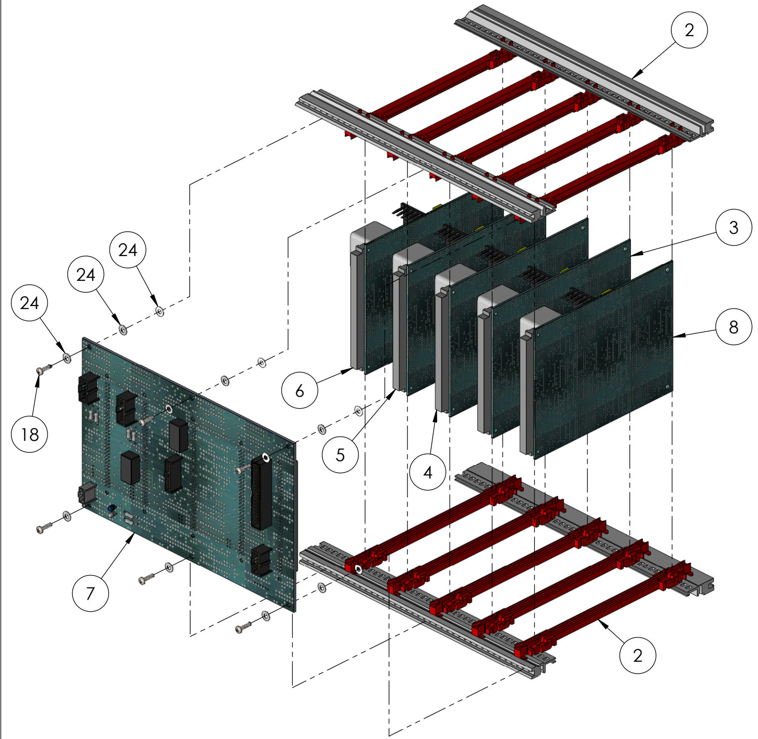
PCB EXPLODED VIEW
