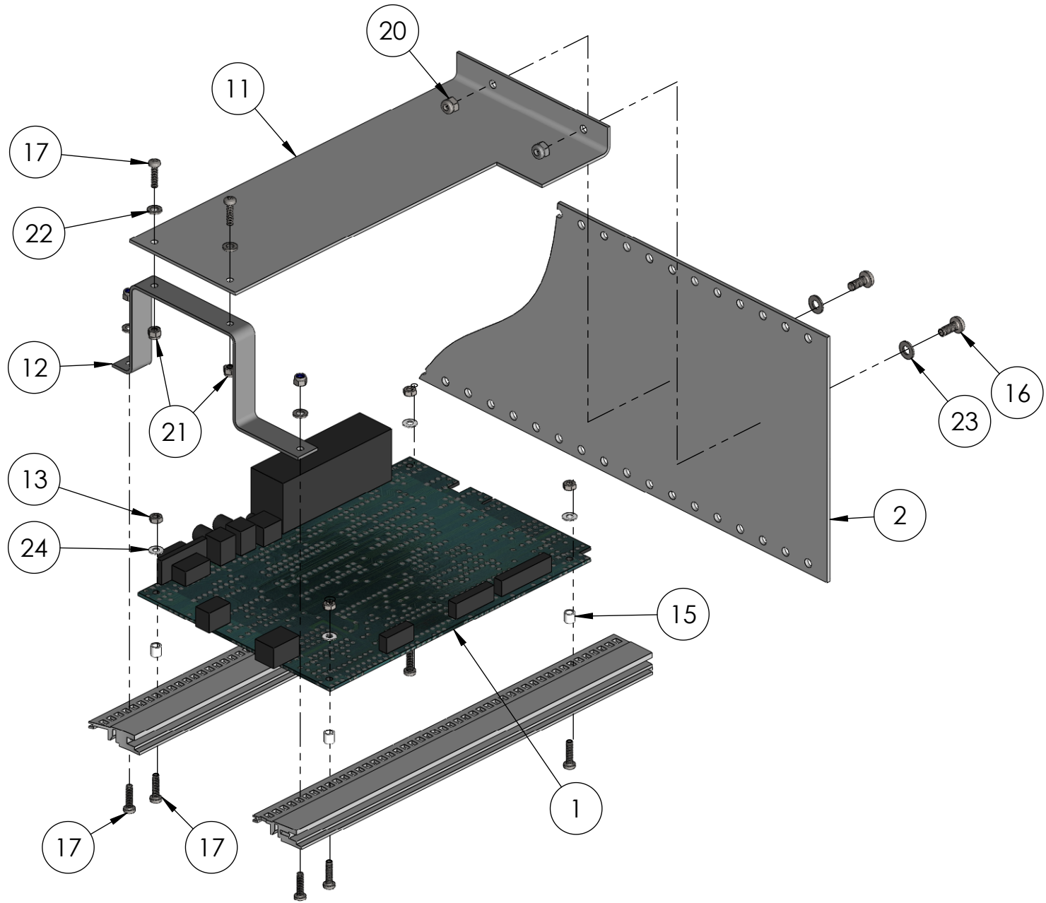
D.S.P. PCB & MOUNTING/PROTECTING COMPONENTS
