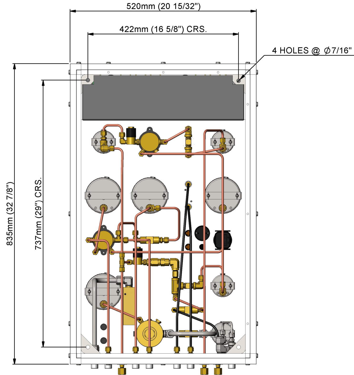
REAR VIEW
