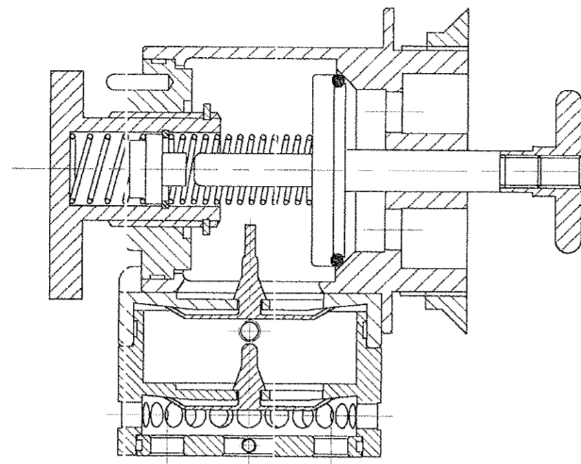
SECTIONAL VIEW
