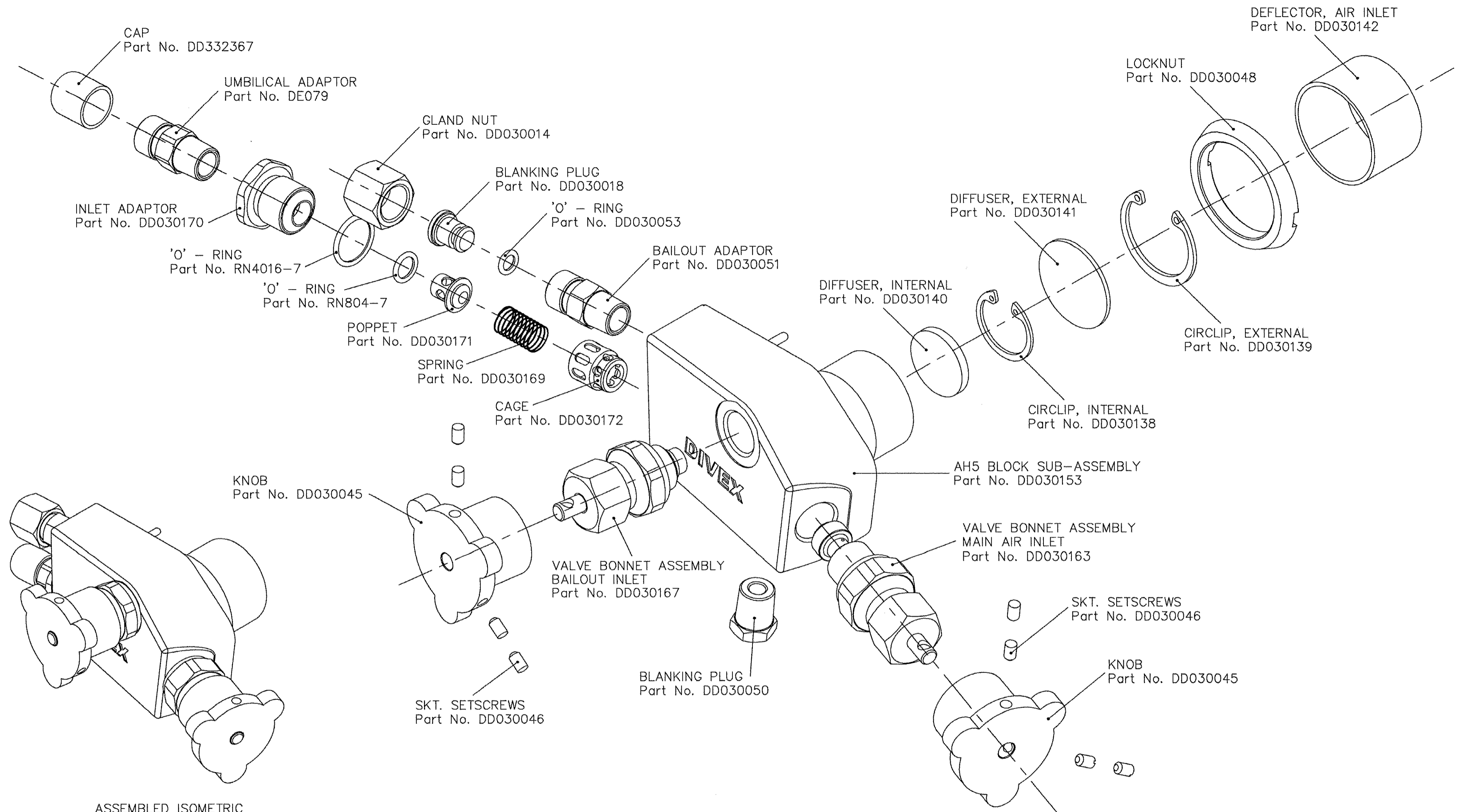
ASSEMBLED ISOMETRIC
