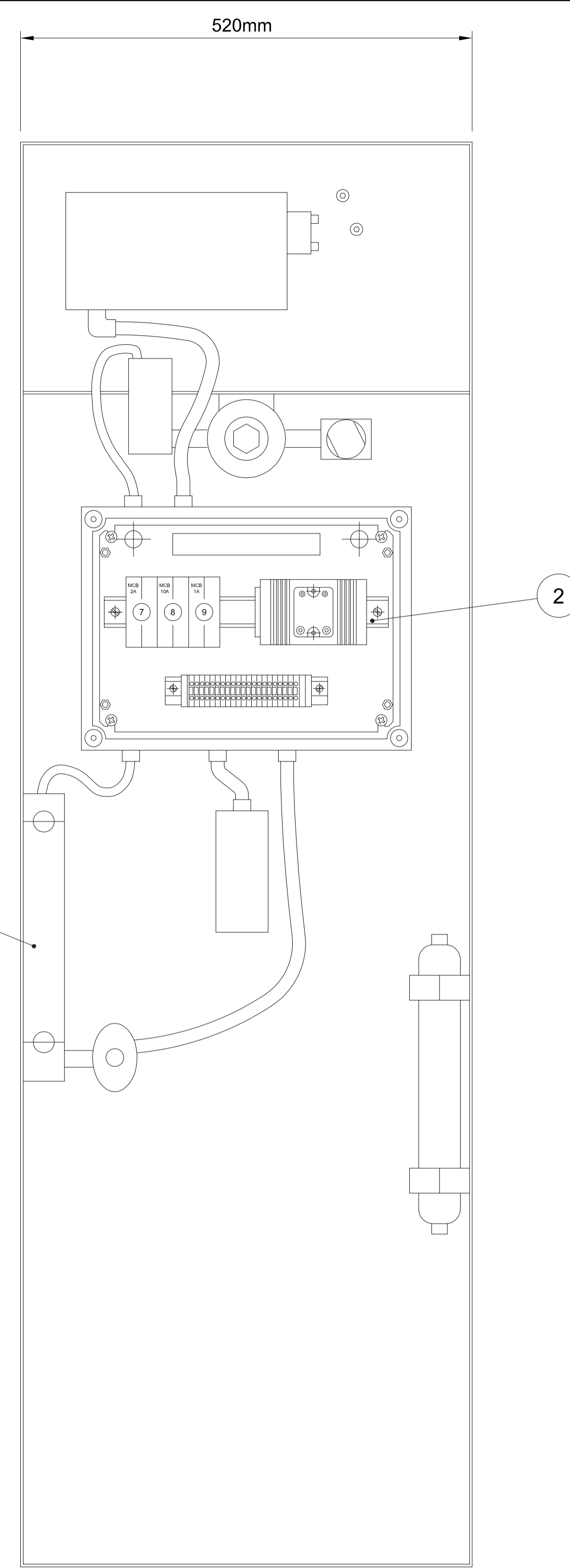
REAR ELEVATION
